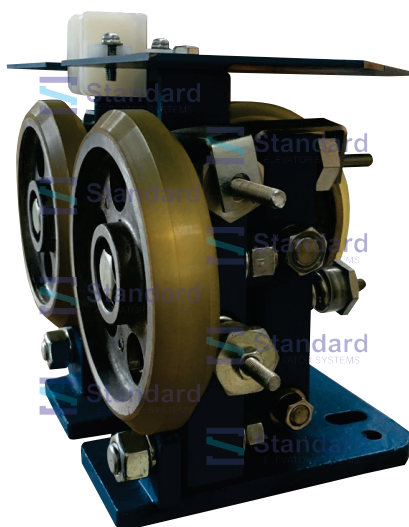
RGS10-273P5
